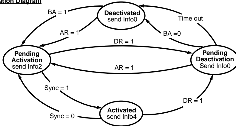
Figure 7 - Link Activation Protocol, State Diagram
