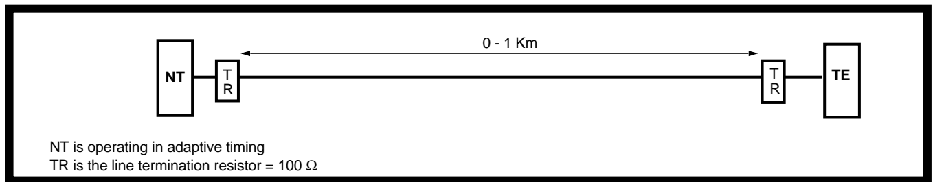
Figure 8 - Point-to-Point Configuration
